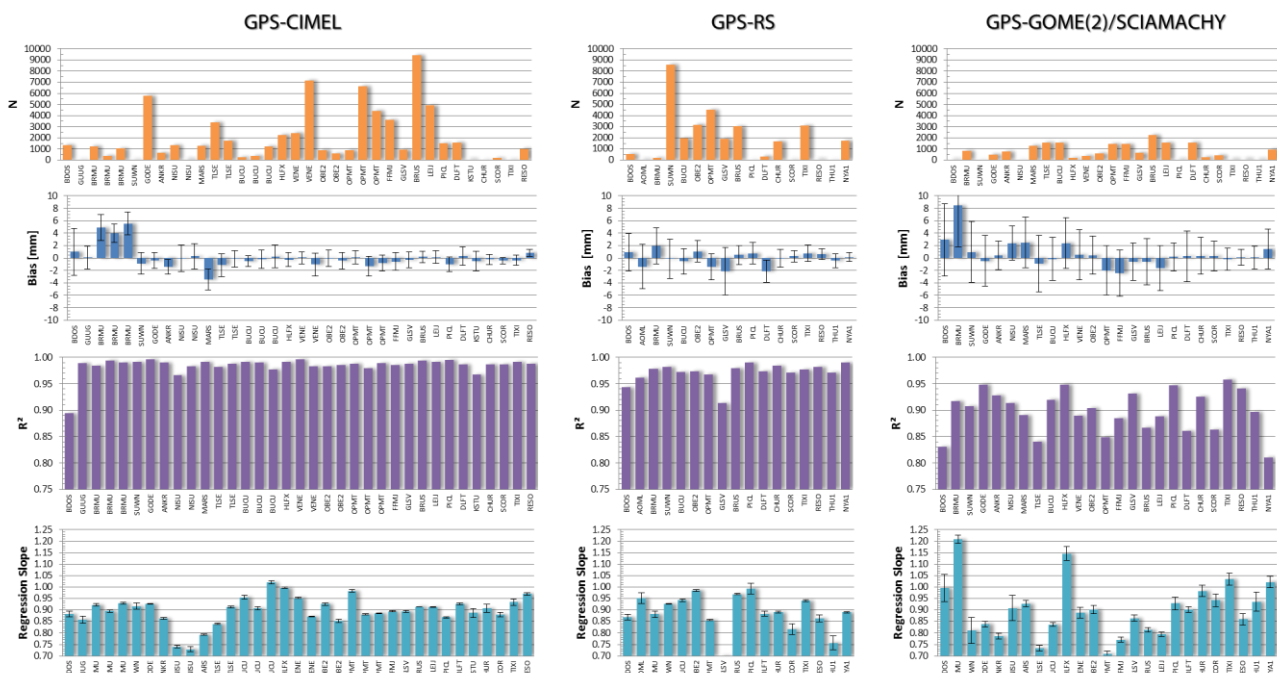
Figure 3: Column bar plots of scatter plot properties (count N , bias, R^2 and regression slope) of the different instruments versus GNSS for the selected sites worldwide. Sites are ordered with increasing latitude. The errors represent the RMS (bias) and the standard deviation (regression slope).
