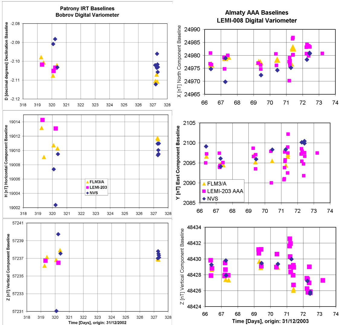
Figure 3. Baselines obtained with CRENEGON Difluxes during intercomparison sessions
